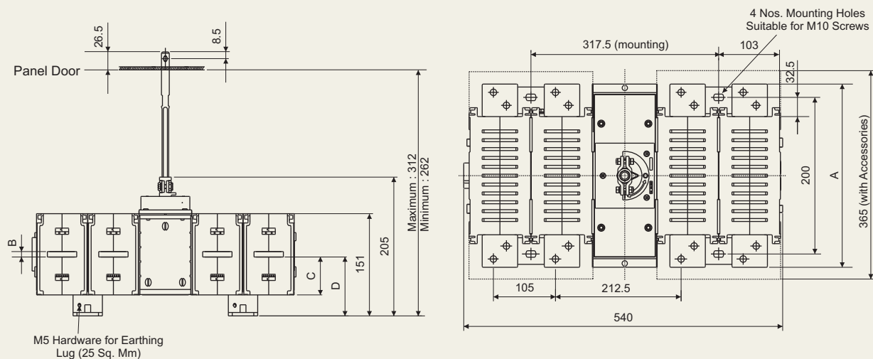
1000/1250 Terminal Arrangement
